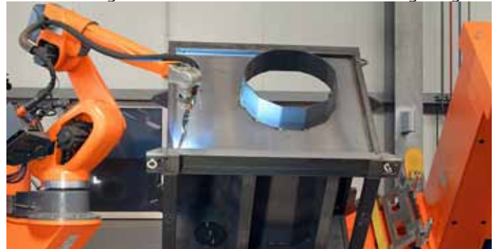
Photo 2: The 1.5-ton workpiece positioner always brings the machine housing into the perfect position for welding.
