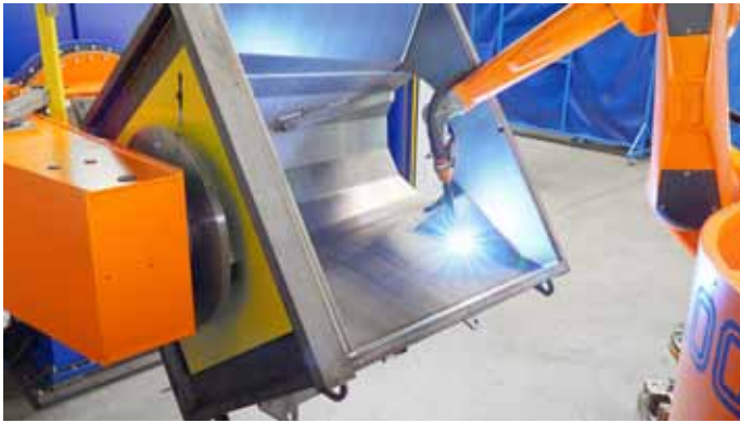
Photo 3: The CLOOS welding robot reaches more than 80 percent of the welds on the complex workpiece.
